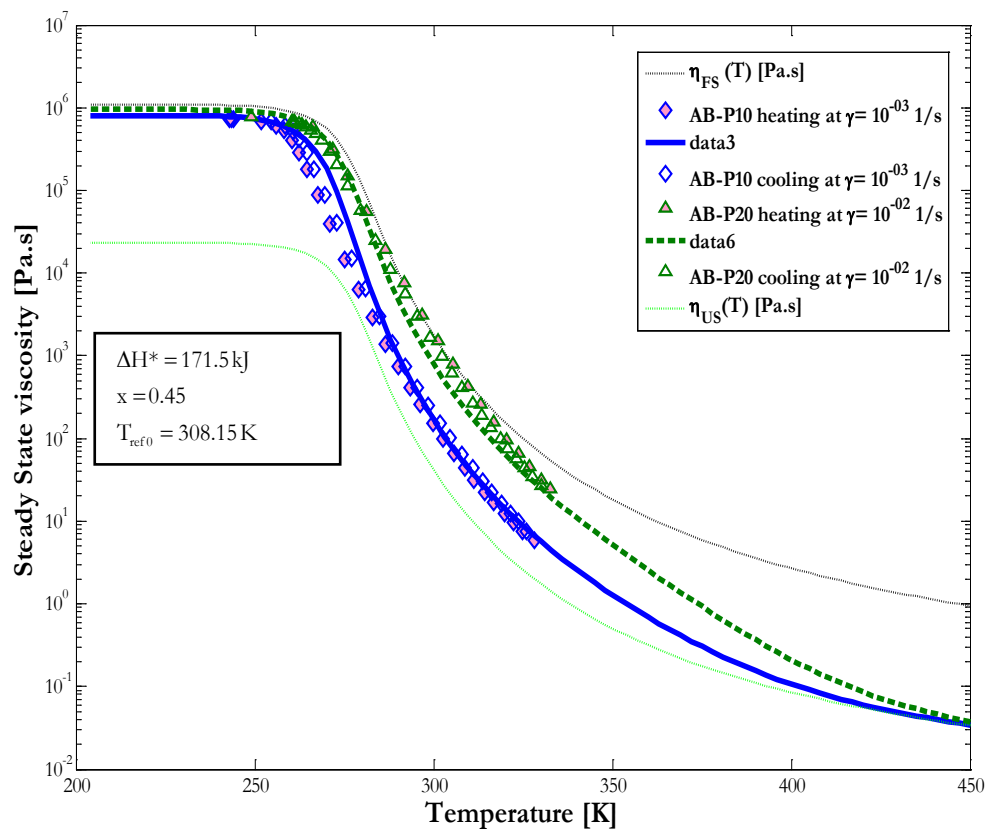
Figure IV.14 : Shear viscosity of Athabasca Bitumen permeates (AB-P10 and AB-P20) at constant shear rate for a temperature sweep. Symbols are experimental; lines are calculated. (Refer to Appendix 2 for the prediction*** data set)
