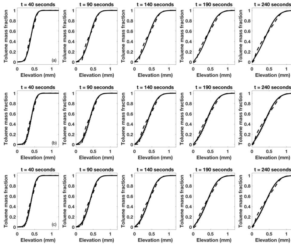
Figure 3.6 Comparison among Fadaie et al. 26 experimental data (dashed), the Fickian diffusion model ( D = 1.6 \times 10^{-10} \text{ m}^2/\text{s} ) (solid) and a Fickian diffusion ( D = 1.6 \times 10^{-10} \text{ m}^2/\text{s} ) + sorption model (dotted) using Langmuir sorption parameters for: a) carbon black, b) activated carbon F300, and c) activated carbon F400.
