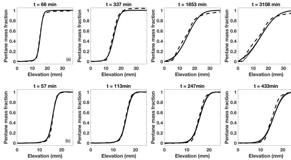
Figure 3.7 Comparison among Athabasca bitumen + pentane 24 (a) and Athabasca atmospheric residue + pentane 24 (b). Experimental data (dashed), a Fickian diffusion only model ( D = 1.6 \times 10^{-10} \text{ m}^2/\text{s} ) (solid) and Fickian diffusion + sorption model ( D = 1.6 \times 10^{-10} \text{ m}^2/\text{s} ) (dotted) based on the properties of activated carbon F300.
