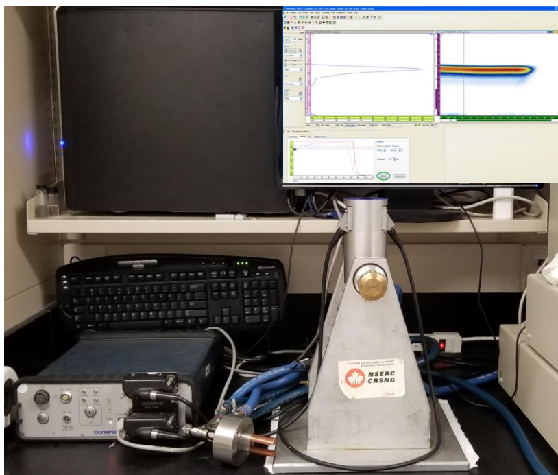
Figure C.1 Acoustic view cell setup
