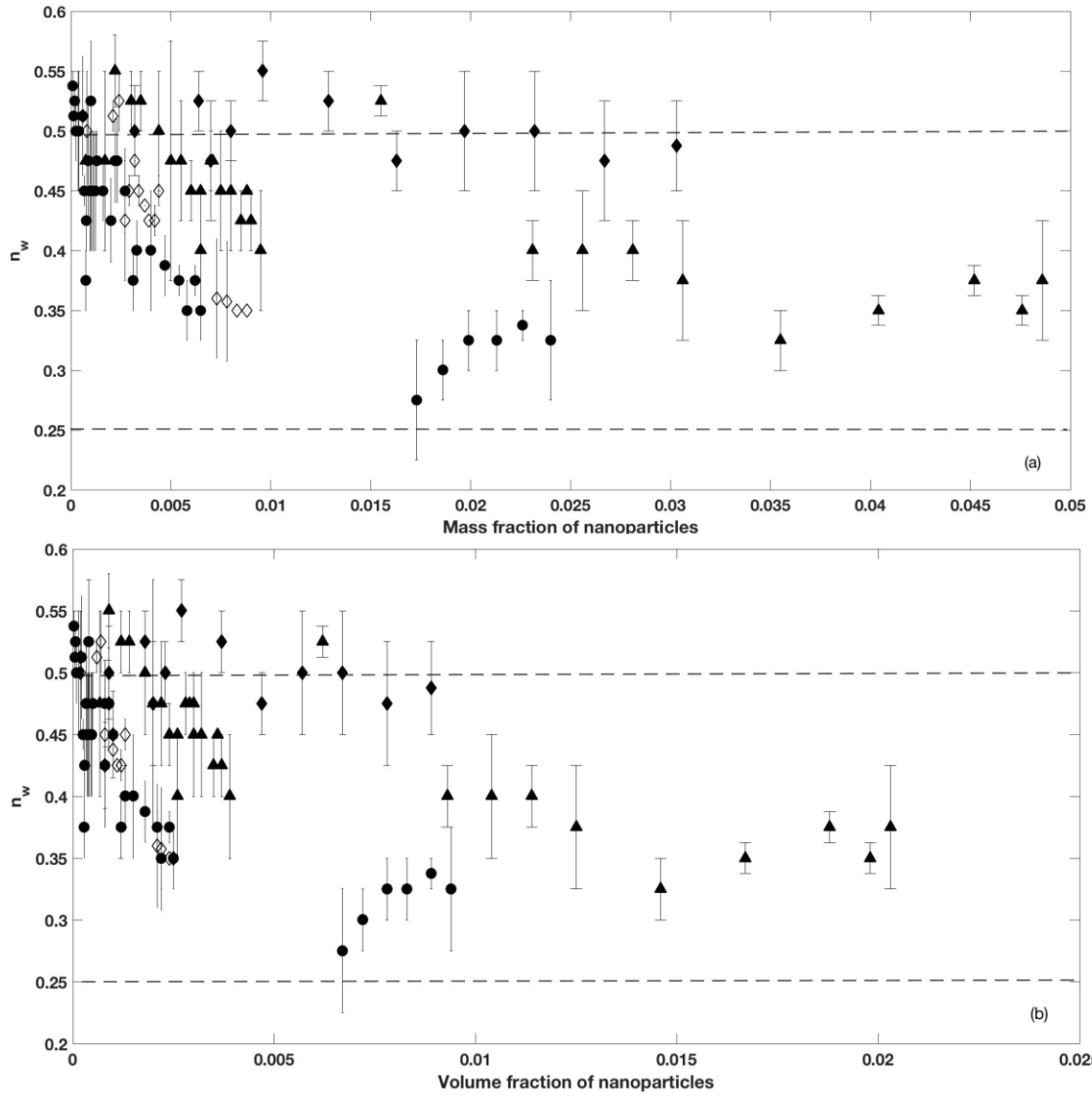
Figure 4.6 Local values of n_w and their uncertainties for carbon nanotubes (▲), 65 nm diamond (◆), 12 nm diamond (◇), and nanosilica (●) at different mass fractions (a) and volume fractions (b) of nanoparticles.
