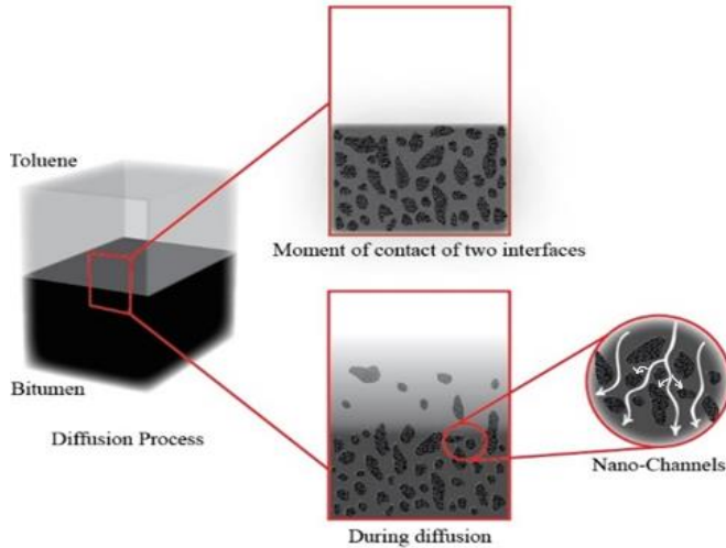
Figure 3.2 Schematic showing mutual diffusion of toluene and bitumen (taken from Alizadehgiashi et al. 20 )
