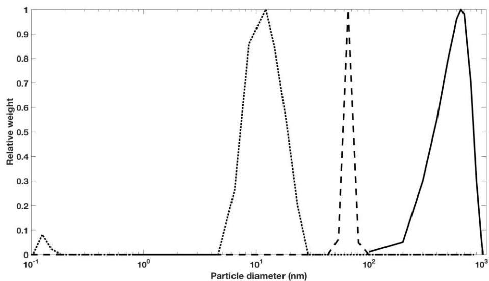
Figure 4.3 Particle size distribution of microdiamond particles before treatment (solid), after first treatment (dashed) and after second treatment with filter (dotted).
