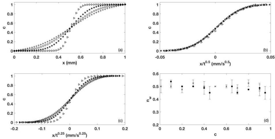
Figure 4.1 Fickian composition profile after 10s ( \triangleright ), 60s ( * ), 120s ( \circ ), and 190s ( + ), plotted against (a) distance, (b) \lambda with n_w = 0.5 , and (c) \lambda with n_w = 0.25 . (d) Uncertainties of values of n_w based on absolute difference ( \blacksquare ) and derivate fits ( \times ).
