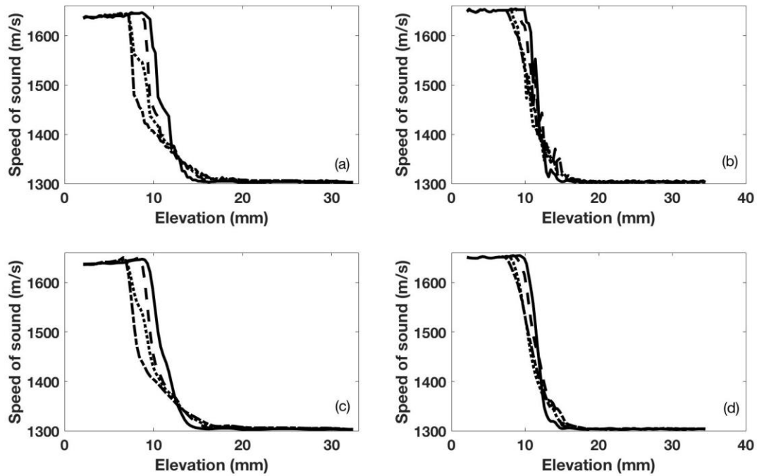
Figure 3.3 Speed of sound profiles for (a) toluene + polybutene (raw data) (b) toluene + (0.05 mass fraction carbon nanotubes + polybutene) (raw data) (c) toluene + polybutene (smoothed data) and (d) toluene + (0.05 mass fraction carbon nanotubes + polybutene) (smoothed data) after 3hr ( — ), 6hr ( ---- ), 9hr ( .... ) and 12hr ( -.-.- ).
