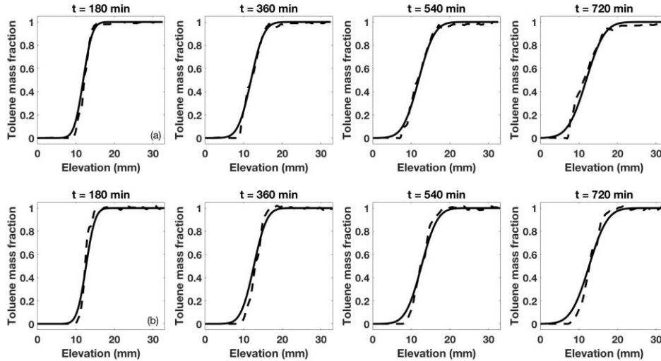
Figure 3.8 Comparison of Fickian diffusion model with D = 1.6 \times 10^{-10} \text{ m}^2/\text{s} (solid line) with experimental data (dashed line) for (a) toluene + polybutene (dashed); (b) toluene + (0.05 mass fraction carbon nanotubes + polybutene)
