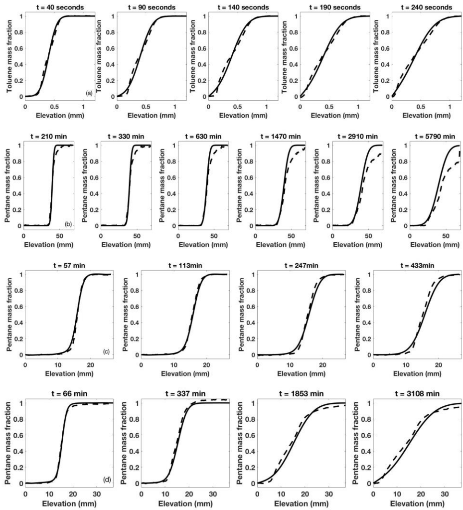
Figure 3.5 Comparison of Fickian diffusion model (solid) with smoothed experimental composition profile data (dashed) for (a) Athabasca bitumen + toluene 26 ; (b) Athabasca bitumen + pentane 22,23 (c) Athabasca atmospheric residue + pentane 24 ; (d) Athabasca bitumen + pentane 24 . D = 1.6 \times 10^{-10} \text{ m}^2/\text{s}
