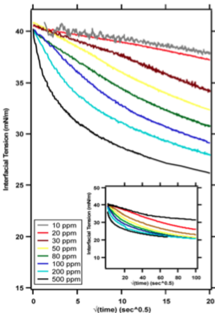
Figure 2.9: Diffusion mechanism identification for asphaltenes at a nexbase 2002/deionized water interface. (Graph from reference 2.50)
