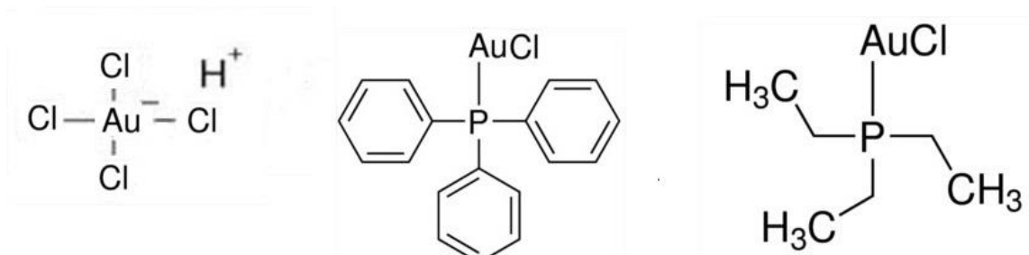
Figure 2.2: Example of gold Salts. Left: \text{H[AuCl}_4\text{]} oxidation state of gold III Center: \text{P(Ph)}_3\text{AuCl} oxidation state of gold I Right: \text{(Et)}_3\text{PAuCl} oxidation state of gold I
