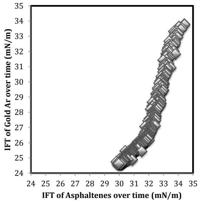
Figure 4.29: Parity plots for the variation of C 5 -Athabasca asphaltenes and gold-Ar nanoparticles in toluene: 500mg/L
