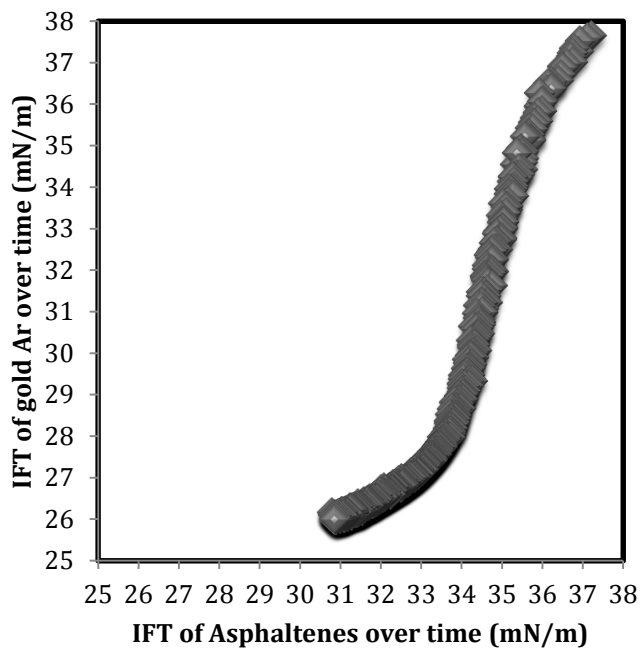
Figure 4.30: Parity plots for the variation of C 5 -Athabasca asphaltenes and gold-Ar nanoparticles in toluene: 1000mg/L
