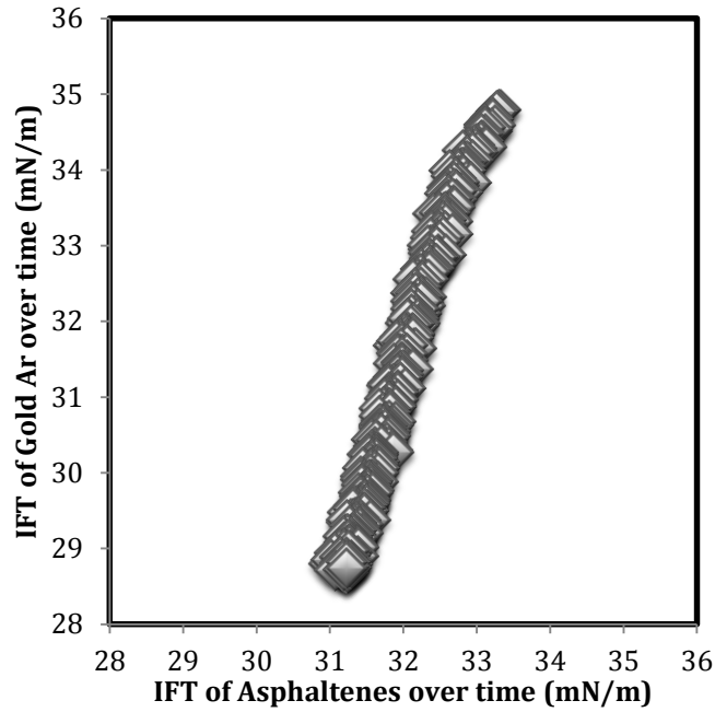
Figure 4.28: Parity plots for the variation of C 5 -Athabasca asphaltenes and gold-Ar nanoparticles in toluene: 100mg/L
