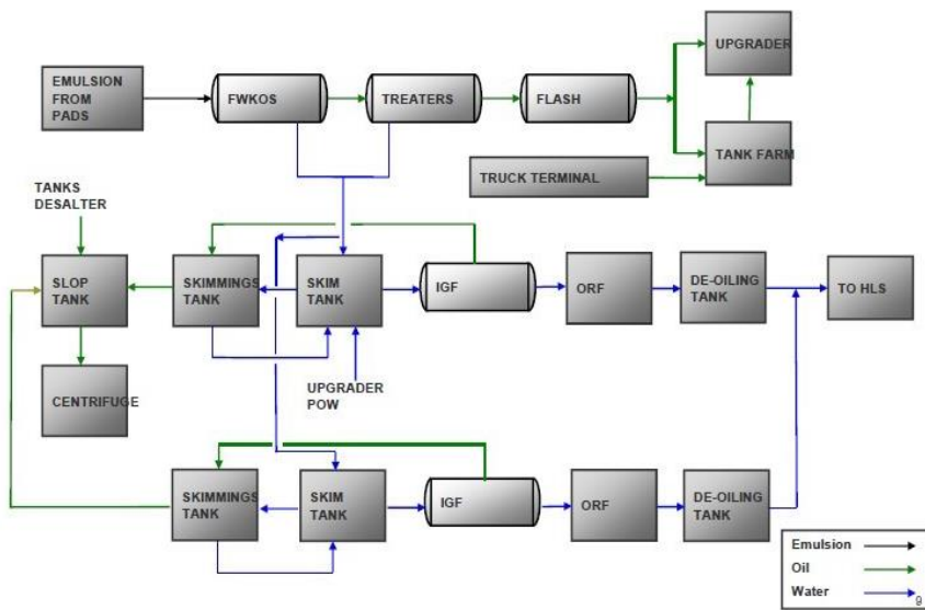
Figure 1-9 Schematic diagram of the Nexen Long Lake SAGD produced water treatment process (before the hot lime softening process) [27]
