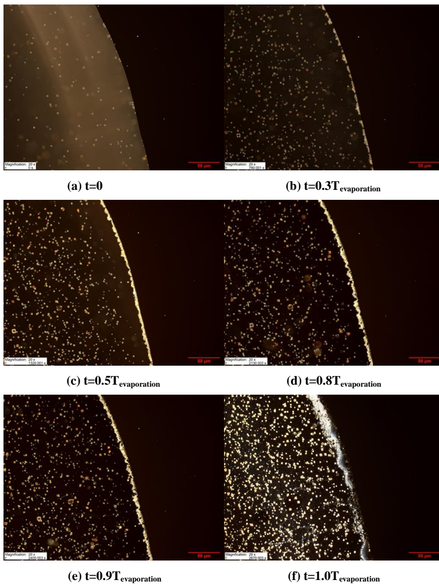
Figure 4-5 A series of images illustrating the growth of liquid crystals at the rim area in a 10 \mu\text{L} sessile drop of the low concentration sample. t is the fraction of the total evaporation time T_{\text{evaporation}} = 2670 seconds for the sessile drop.
