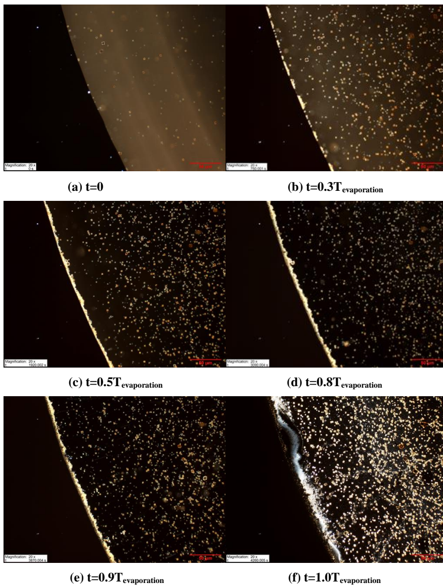
Figure 4-6 A series of images illustrating the growth of liquid crystal domains at the rim area in a 30 \mu\text{L} sessile drop of the low concentration sample. t is the fraction of the total evaporation time T_{\text{evaporation}} = 4260 seconds for the sessile drop.
