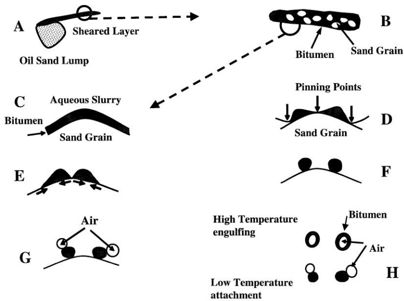
Figure 1-15 Illustration of the bitumen liberation and aeration [11]
