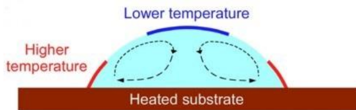
Figure 4-2 A Marangoni flow pattern in an evaporating drop on a heated substrate [64]
