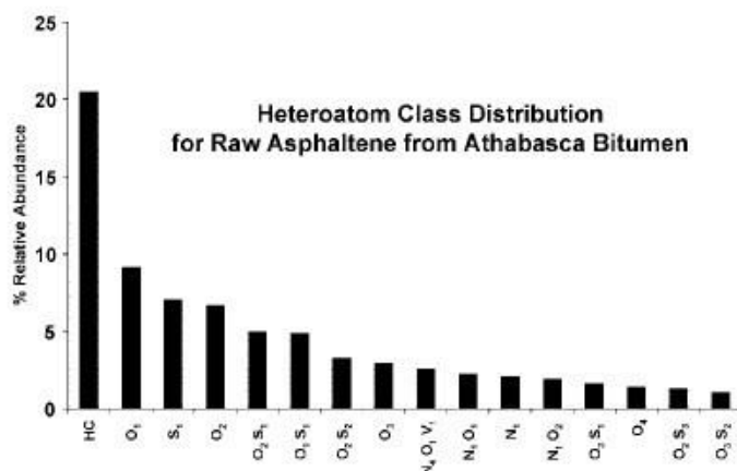
Figure 1-5 Heteroatom abundance distribution for Athabasca C 7 asphaltenes [10]
