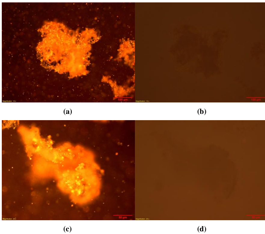
Figure 3-6 Microscopic observation of flocs in the aged Nexen FWKO subsample A:(a) under cross polarized light, magnification 10x; (b) under normal light, magnification 10x; (c) under cross polarized light, magnification 20x; (d) under normal light, magnification 20x.
