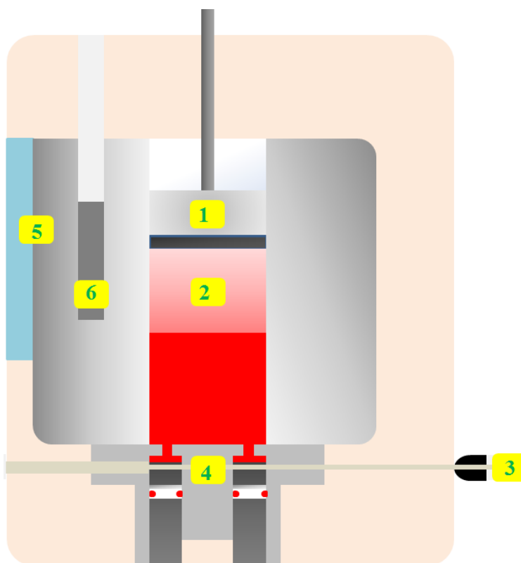
Figure 3.1 Cross-section view of the measuring cell: 1) pressure transducer 2) measuring chamber 3) Luer sample inlet 4) sample inlet valve 5) thermoelectric module 6) PT100 RTD sensor, adapted from the operation manual. 1
